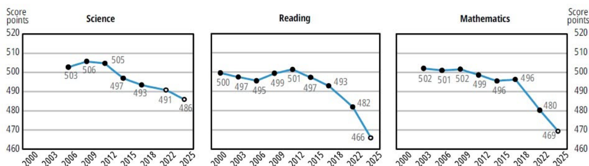
Figure I.2.6. Trends in performance over time in science, reading and mathematics
